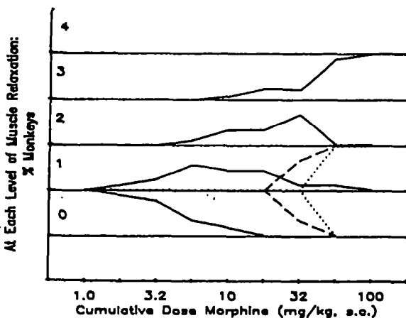
FIGURE 2. The effect of cumulative morphine alone (solid lines) and after 24-hr (dashed lines) or 46-hr (dotted lines) pretreatment with 10 mg/kg \beta -FNA on muscle relaxation in normal monkeys (n=6).
