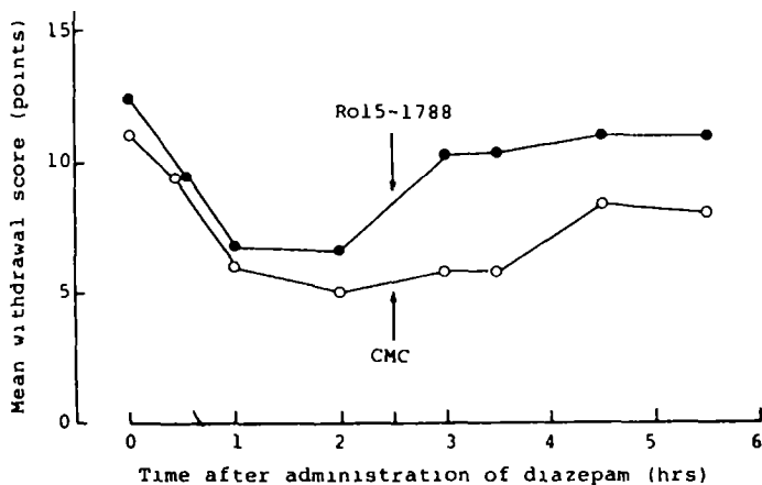
FIGURE 1 Diazepam 4 mg/kg was administered about 50 hours after the last dose of barbital and 2.5 hr later, Ro15-1788 (●) and control (CMC) (○) were administered to 3 monkeys each. The barbital withdrawal signs suppressed by diazepam were precipitated by the benzodiazepine antagonist.
