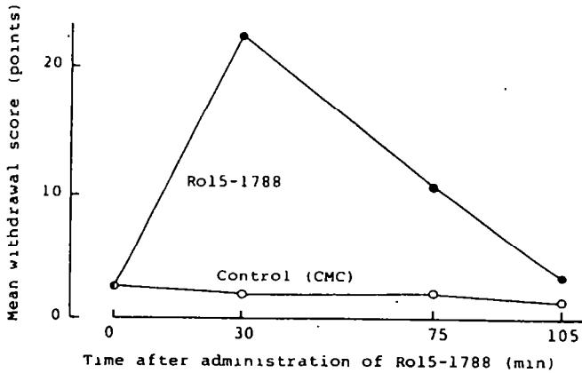
FIGURE 2 Rol15-1788 (●) and control (CMC) (○) were administered to respective 4 and 2 diazepam-dependent monkeys 2.5 hours after the last diazepam dose. The antagonist precipitated the diazepam withdrawal signs.
