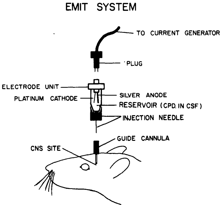
Figure 1. The electrolytic microinfusion transducer system used for intracranial administration and self-administration experiments (from Goeders et al. 1984) Copyright 1984, Ankho International Inc.
