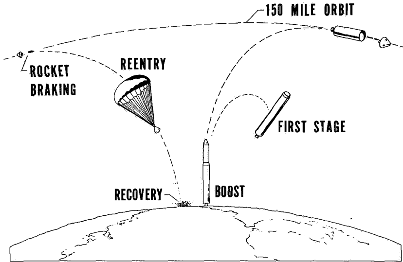
A diagram used at the first NASA inspection to illustrate the basic concept of a Mercury man-in-space mission.
