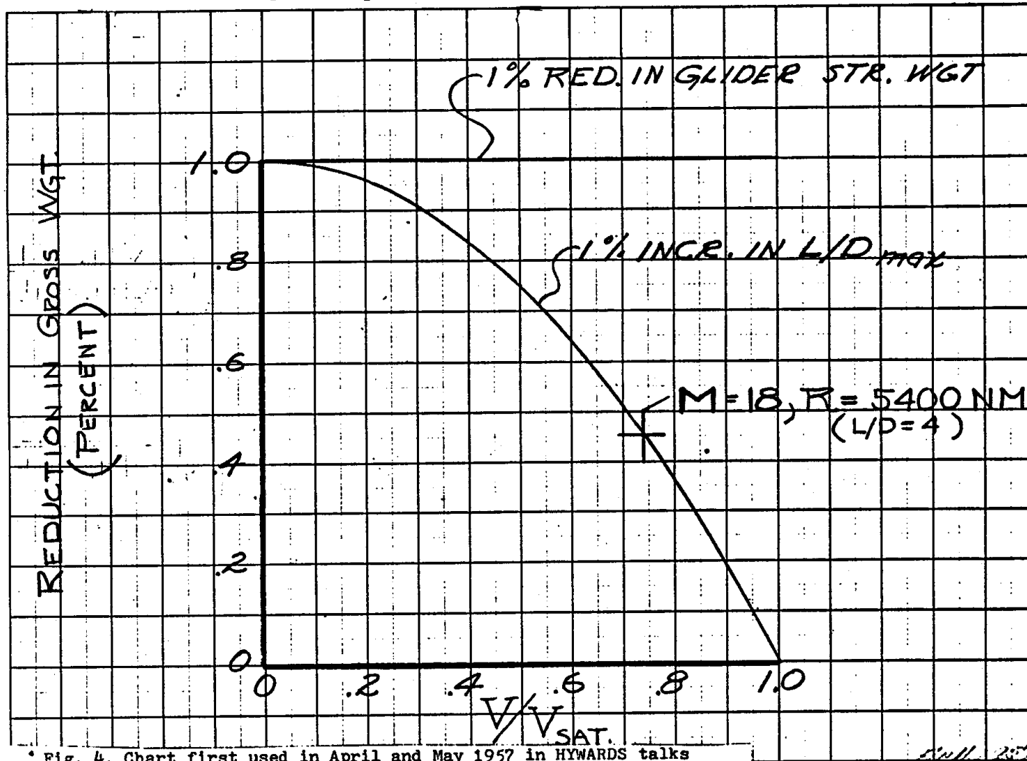
* Fig. 4. Chart first used in April and May 1957 in HYWARDS talks at Langley to show the decreased relative importance of L/D at high hypersonic speeds, and the constant importance of structural weight.
