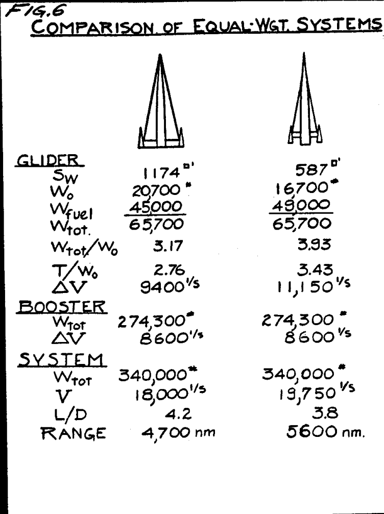
Fig. 6. Chart used in Round III summary talk by J.V. Becker showing how the Langley glider could achieve increased range by L/D reduction through use of a smaller wing, and emphasizing the need for optimization analyses of both the Ames and Langley vehicles. Ref 14.
