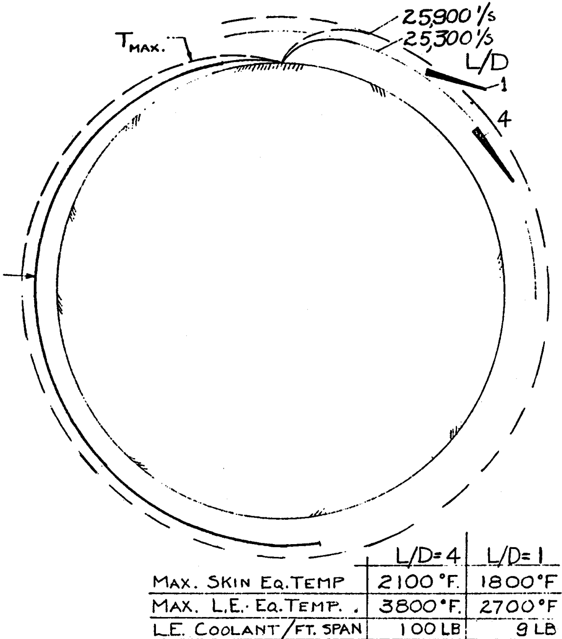
Fig. 5. Langley chart dated May 1, 1957, extending the idea of high-angle-of-attack operation to maximum lift 60-45° ( L/D \sim 1 ) for global-range flights. Most of the range is covered on the outer fringe of the atmosphere at low heating rates; peak deceleration and heating occur near the end of the trajectory. Skin temperatures and coolant requirements greatly reduced in comparison to the high- L/D flight.
