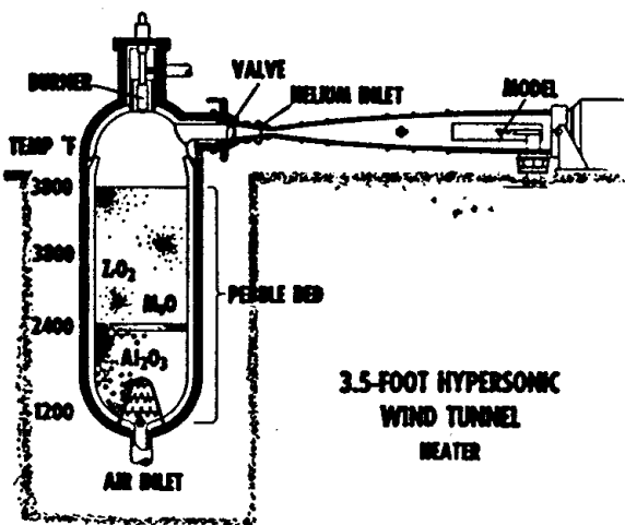
NACA AMES 3.5 ft. HYPERSONIC WIND TUNNEL
