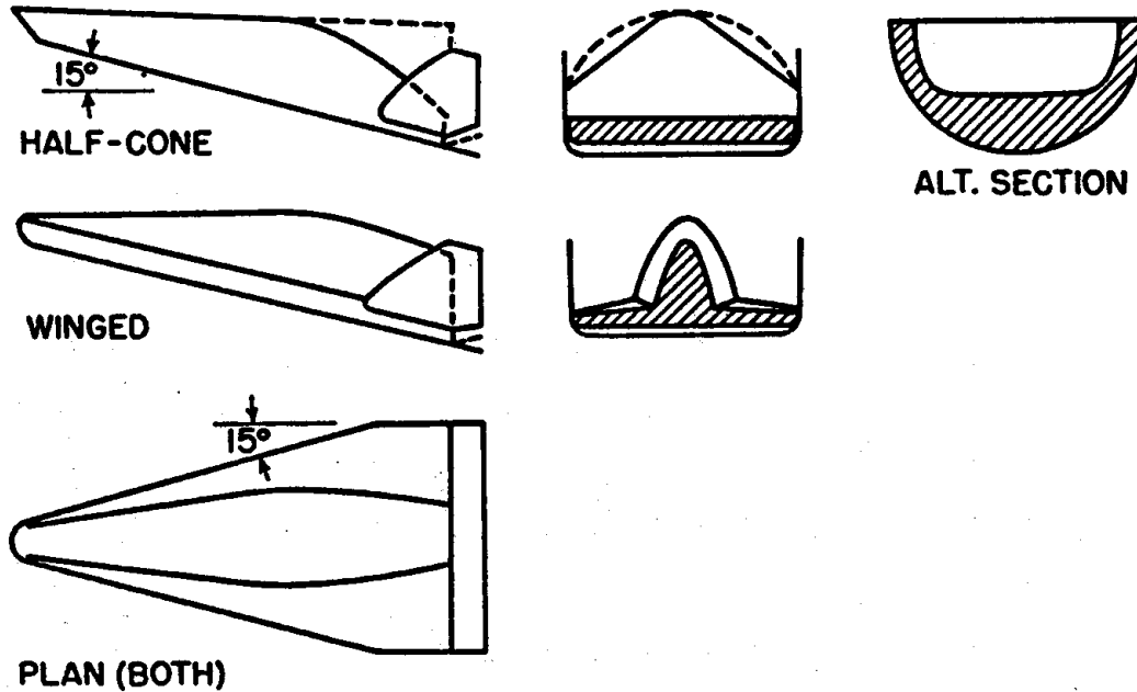
Fig.12. Chart used in NASA presentation at SAB meeting of Dec.2-4 to compare the conceptual Dyna-Soar wing-body with comparable lifting bodies of the same platform. Data were available for wing-bodies indicating L/D 2, hypersonic, and 5, subsonic. The lesser performance of the lifting bodies was estimated as approximately L/D 1.5, hypersonic, and 3, subsonic.
