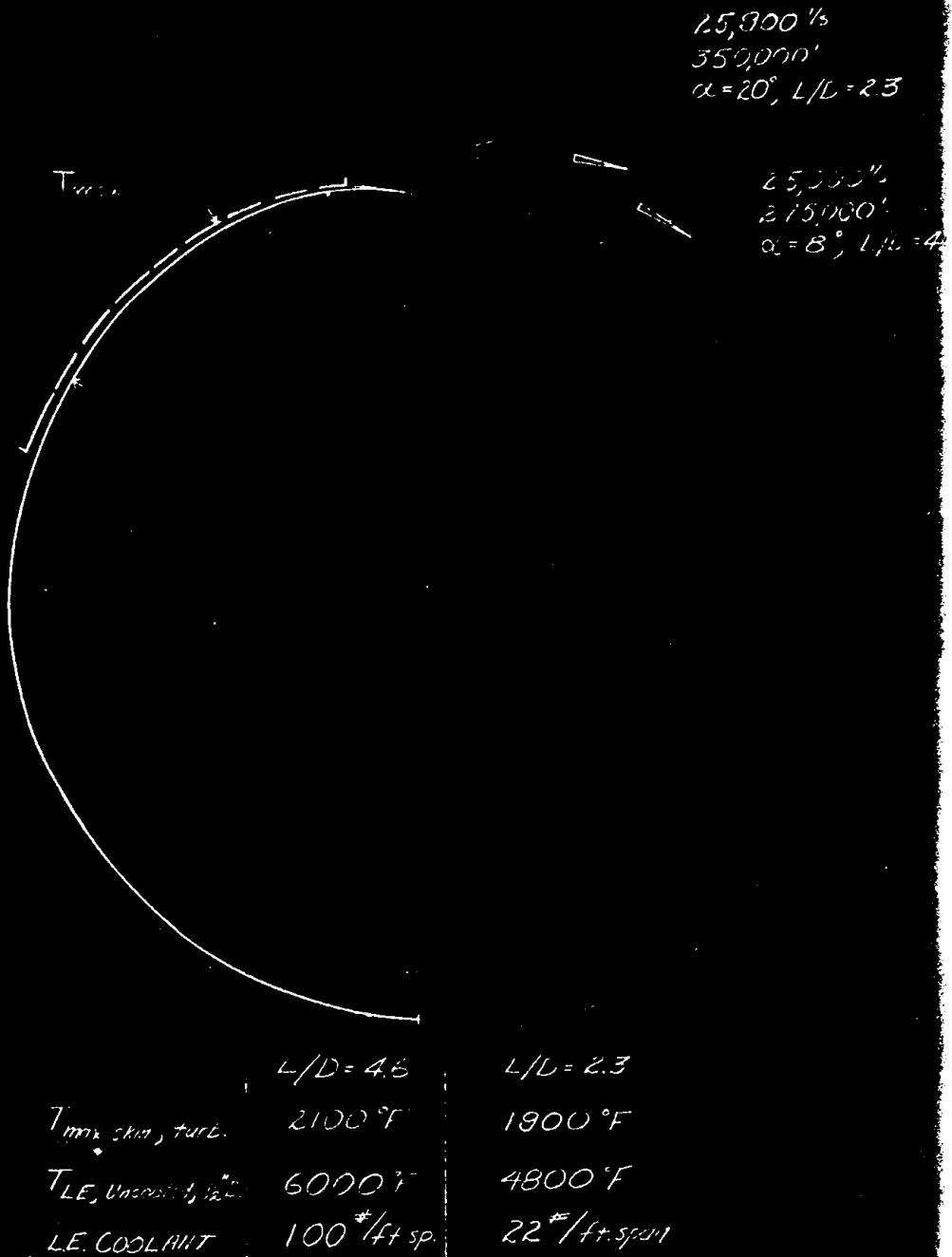
Fig. 2. Chart developed in Langley HYWARDS study for presentation to Langley management on Jan.11,1957, showing heating alleviation for global-range glides by operation at high angle of attack and reduced L/D. (See Ref.8)
