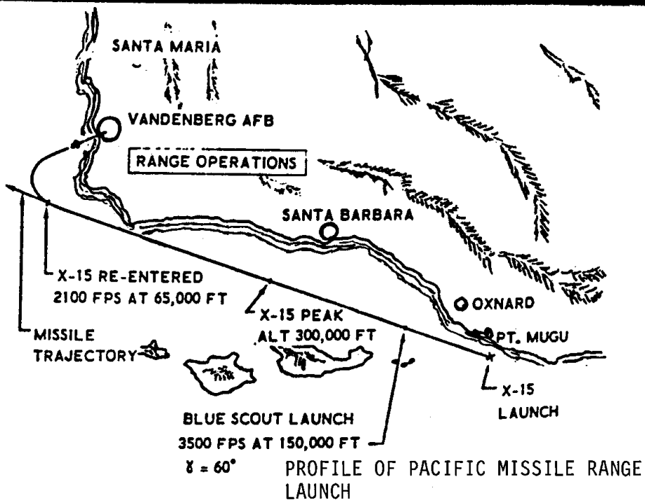
X-15/Blue Scout Launch System
